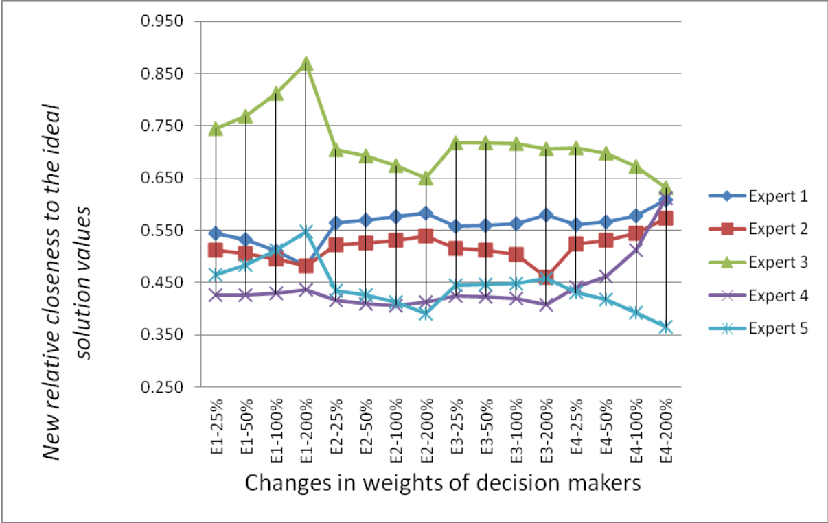
Figure 4. Sensitivity analysis of the Decision Maker weights.
