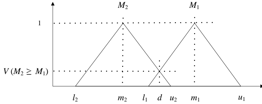
Figure 2. Intersection point “d” between two fuzzy numbers M_1 and M_2 .
