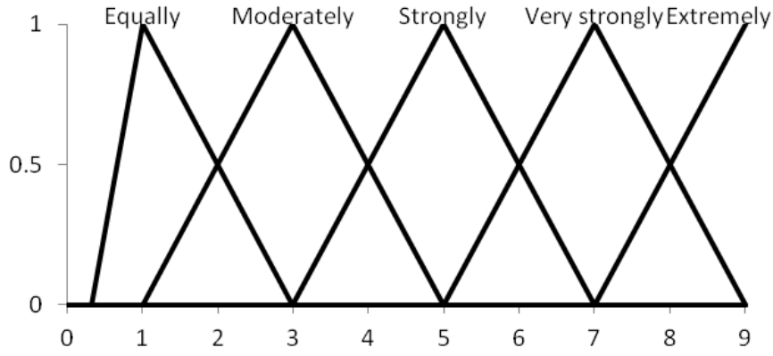
Figure 1. Linguistic variables and membership function of each criterion.
