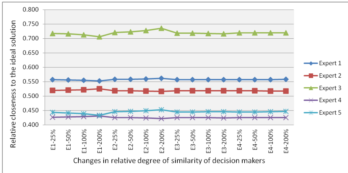
Figure 3. Sensitivity analysis of the decision maker’s relative degree of similarity.
