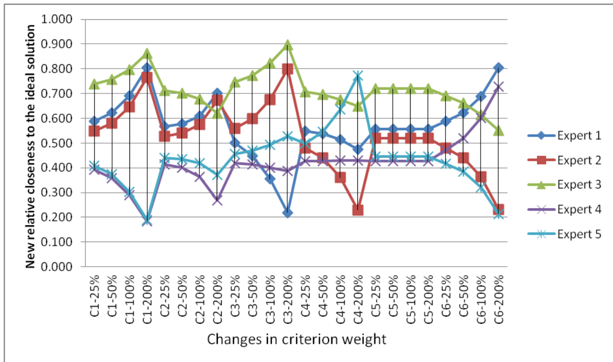
Figure 5. Sensitivity analysis of the criteria weights.
